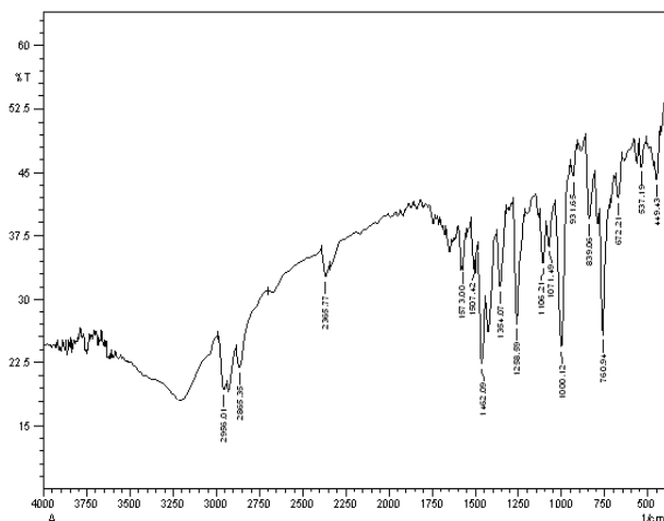
Figure 1: Infrared Spectrum of pure Losartan potassium
