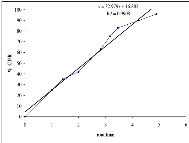
Figure 11: Higuchi matrix release kinetics of optimized formulation (F4)
