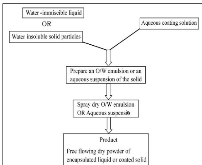
Figure 1: Flowchart for coating liquid and solid particles using spray-dry process
