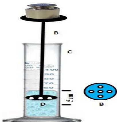
Figure 3: Gel strength measuring device.
